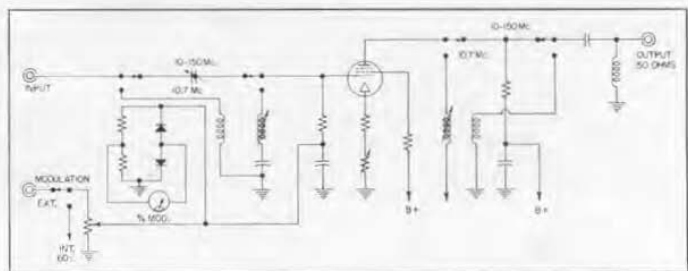
Figure 3. Elementary schematic diagram of the Amplitude Modulator.
