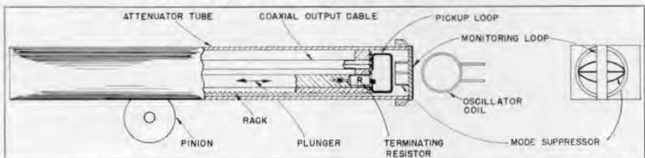
Figure 3. Cutaway view of the attenuator and termination.
